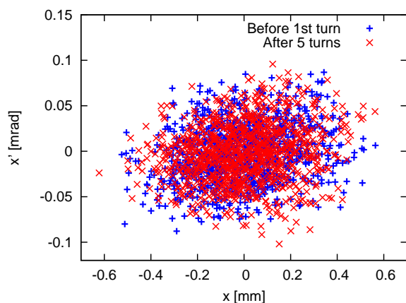
Figure 4: DIMAD tracking results at the 1.5 GeV IP showing the effect of the PSM in single-turn injection mode on the stored beam ( \epsilon_x = 6 \text{ nm rad} , \sigma_\delta = 7.5 \times 10^{-4} , Gaussian distribution with cut-off at 3\sigma ).
