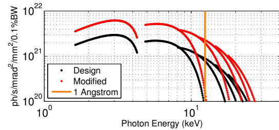
Figure 4: Beyond a two-fold brightness increase at 1 Å (at the 7th harmonic) from the modified optics compared to the design optics in the MAX IV 3 GeV storage ring.
