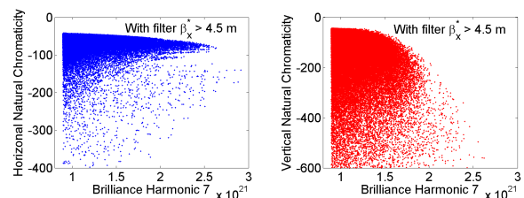
Figure 5: GLASS solutions showing the resulting natural chromaticity and brightness. The design lattice corresponds to the upper left corner in both plots.
