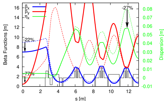
Figure 6: Machine functions for one half of an achromat of the MAX IV 3 GeV storage ring. The design optics are indicated in dashed lines, while the solid lines indicate the modified optics.
