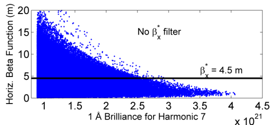
Figure 2: GLASS solutions showing that maximizing brightness requires reducing the horizontal beta function in the long straights \beta_x^* .
