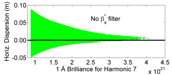
Figure 3: GLASS solutions showing that maximizing brightness requires a small amount of dispersion leaked into the long straights \eta_x^* .
