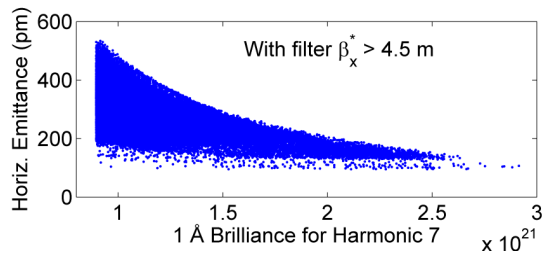
Figure 1: GLASS solutions showing that maximizing brightness requires minimizing bare lattice emittance.
